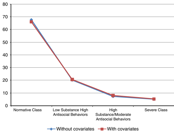
Fig. 5. Probability of four latent classes with and without covariates.
